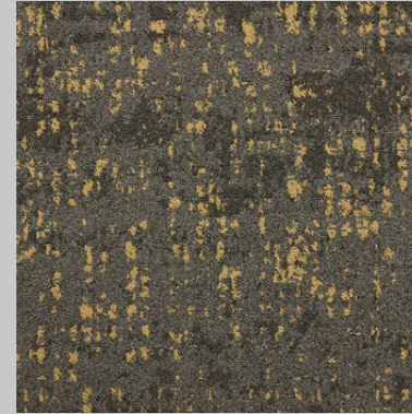
Nebula
