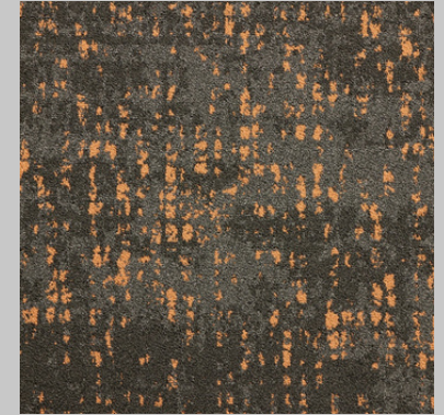
Saturn
