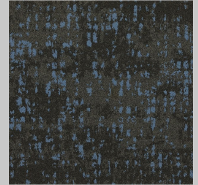
Neptune
